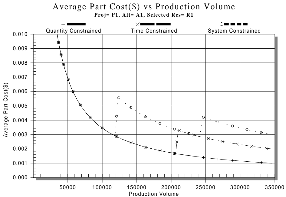
Figure 2. RCM - cost analysis for an individual resource
