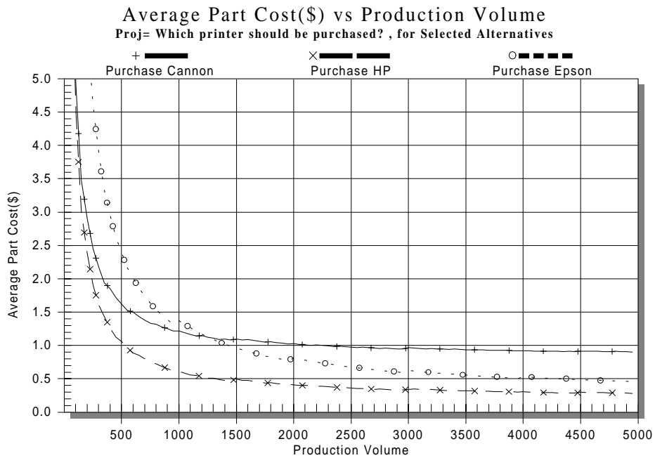
Figure 4. RCM - cost comparison of alternatives
